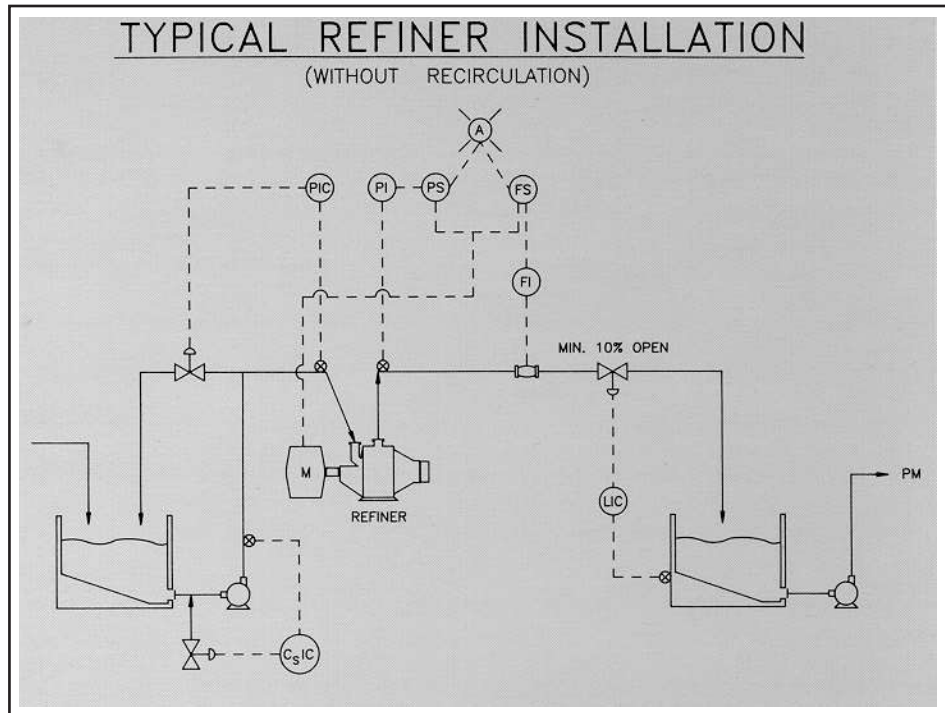
Fig. 1: Single refiner without recirculation
