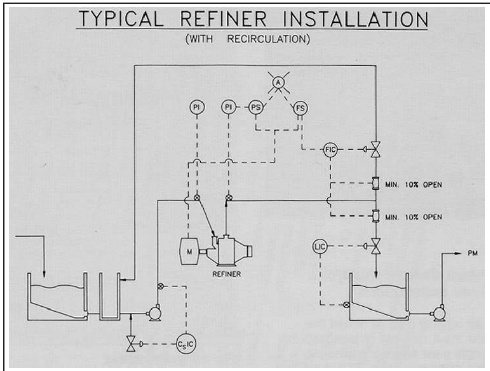
Fig. 2: Single refiner with recirculation
