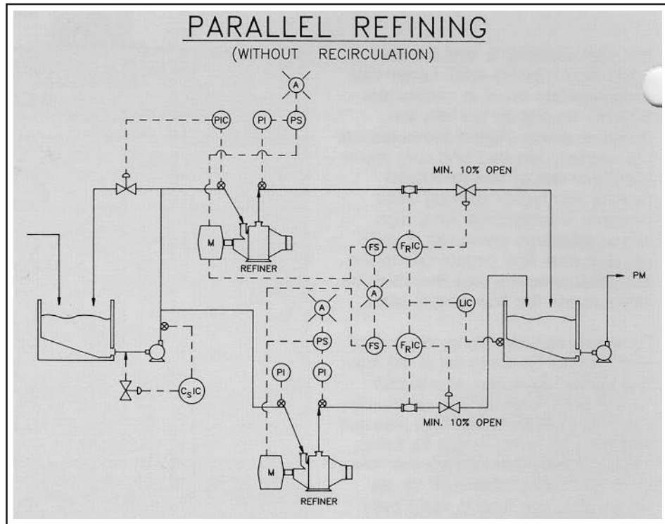
Fig. 4: Parallel refining
