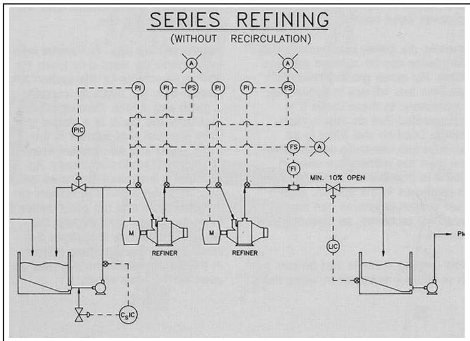
Fig. 3: Series refining
