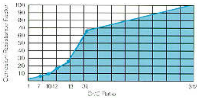
Fig. 5 Corrosion Resistance vs. Chrome/Carbon Ratio
