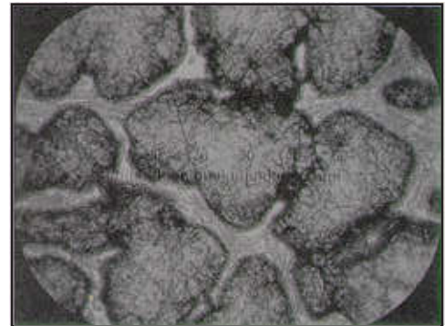
Figure 2. Microstructure of a stainless steel plate. (400x magnification.)
